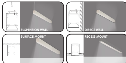
Various mounting options are available from Cable Suspension, Direct Ceiling Surface, Direct Wall Surface and Recessed Ceiling Mounting.
